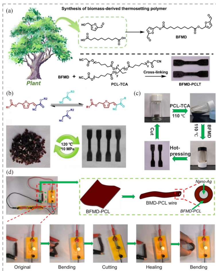
Fig. 5 (a) Solvent-free and catalyst-free dynamic Knoevenagel condensation reaction and the preparation of biomass thermosetting polymers (BFMD-PCL); (b) Re-processability of BFMD-PCL at 120 °C and 10 MPa; (c) Chemical recycling and remolding process of BFMD-PCL; (d) Preparation of BFMD-PCL as a self-healing wire; The conductivity of the wire remains unaltered even after bending, but the light bulb goes out after the wire is cut. Upon heating, the conductive wire undergoes self-healing, and the healed conductive wire retains conductivity even after bending (Reprinted with permission from Ref. [65]; Copyright (2025) the Royal Society of Chemistry).
